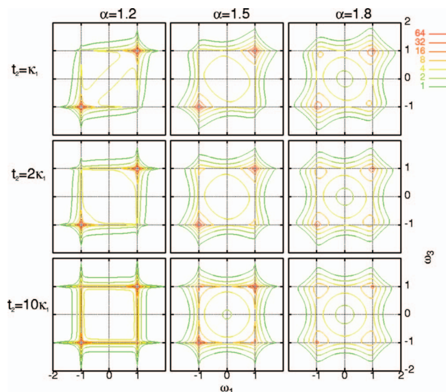
FIG. 7. (Color) The S_A signal [Eq. (15)] for the WTDF [Eq. (33)] for (left to right) \alpha=1.2, 1.5, 1.8 , and \kappa_A/\kappa_1=0.25 , \Omega_0\kappa_1=2.0 , t_2=\kappa_1 (top), t_2=2\kappa_1 (middle), t_2=10\kappa_1 (bottom).
