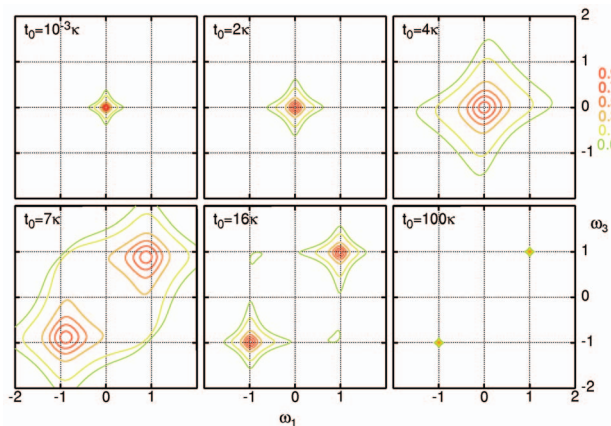
FIG. 10. (Color) Aging 2D Markovian lineshape [Eq. (48)] for various initial times t_0=10^{-3}\kappa , 2\kappa , 4\kappa , 7\kappa , 16\kappa , and 100\kappa . Master equation for probability densities corresponds to the random walk of Fig. 8.
